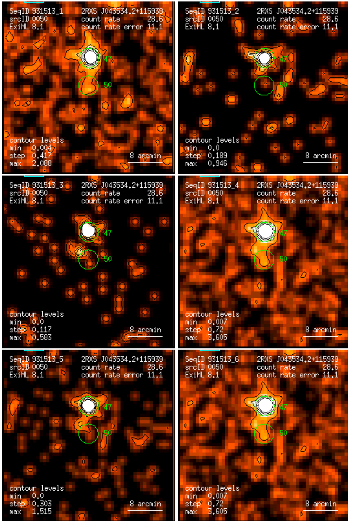
Figure 50: RASS 931513: detection 0050: band rate images, Gaussian filter: (1) PSPC channels 11 – 41, (2) 52 – 90, (3) 91 – 201, (4) 11 – 235, (5) 52 – 201, (6) 11 – 201. Broad band rates in counts/ks. Band rate contour levels in counts/ks/arcmin 2 .
