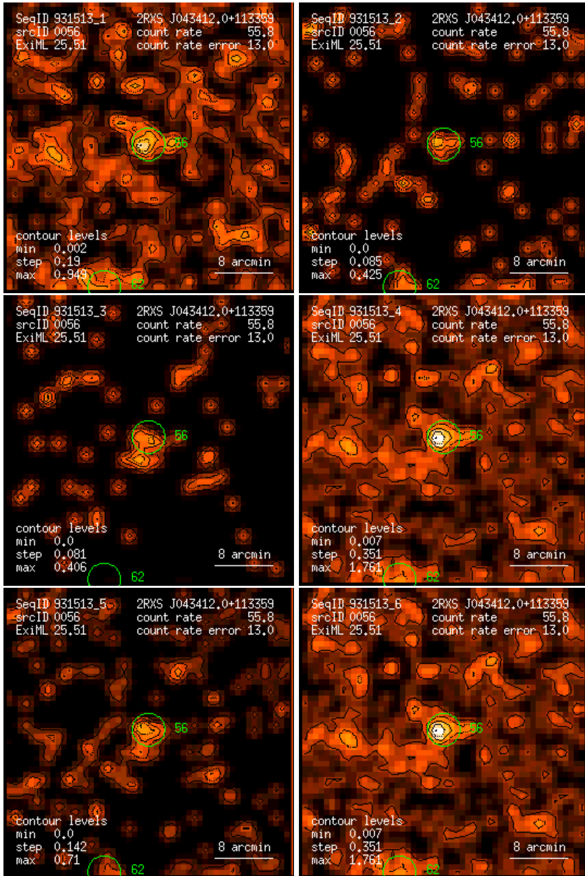
Figure 56: RASS 931513: detection 0056: band rate images, Gaussian filter: (1) PSPC channels 11 – 41, (2) 52 – 90, (3) 91 – 201, (4) 11 – 235, (5) 52 – 201, (6) 11 – 201. Broad band rates in counts/ks. Band rate contour levels in counts/ks/arcmin 2 .
