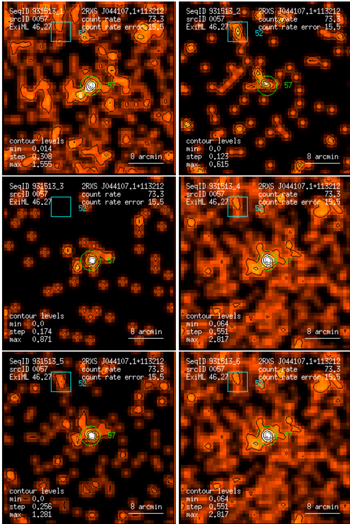
Figure 57: RASS 931513: detection 0057: band rate images, Gaussian filter: (1) PSPC channels 11 – 41, (2) 52 – 90, (3) 91 – 201, (4) 11 – 235, (5) 52 – 201, (6) 11 – 201. Broad band rates in counts/ks. Band rate contour levels in counts/ks/arcmin 2 .
