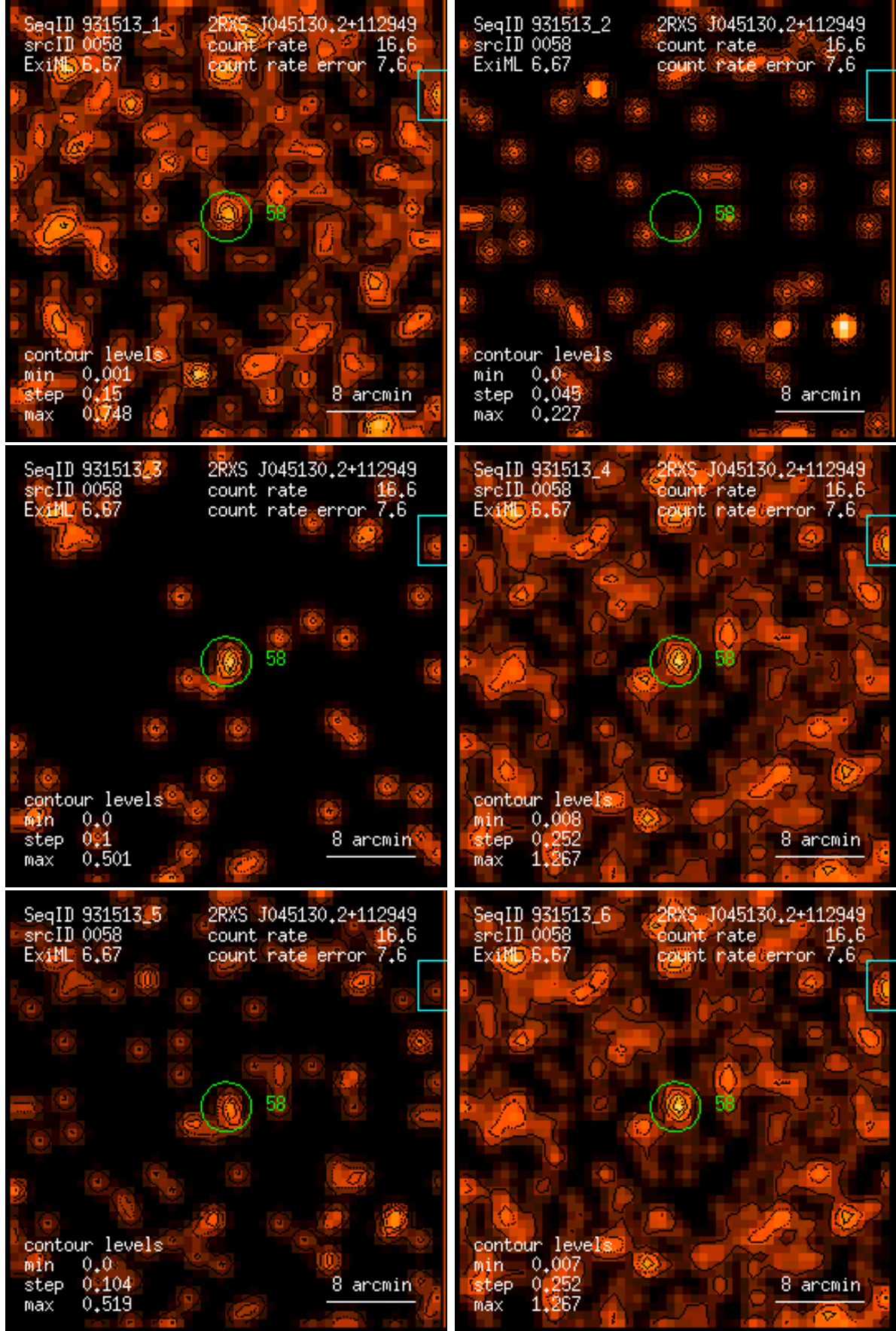
Figure 58: RASS 931513: detection 0058: band rate images, Gaussian filter: (1) PSPC channels 11 – 41, (2) 52 – 90, (3) 91 – 201, (4) 11 – 235, (5) 52 – 201, (6) 11 – 201. Broad band rates in counts/ks. Band rate contour levels in counts/ks/arcmin 2 .
