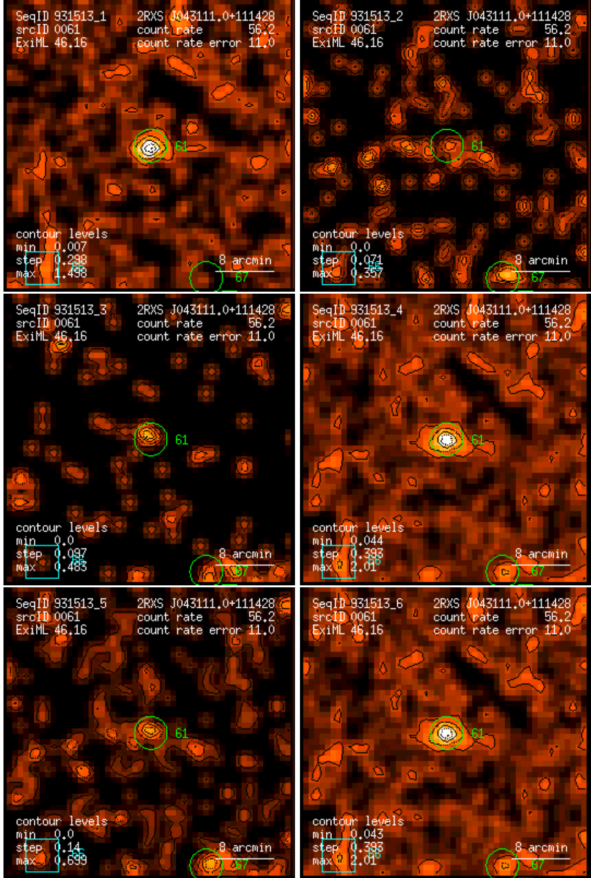
Figure 61: RASS 931513: detection 0061: band rate images, Gaussian filter: (1) PSPC channels 11 – 41, (2) 52 – 90, (3) 91 – 201, (4) 11 – 235, (5) 52 – 201, (6) 11 – 201. Broad band rates in counts/ks. Band rate contour levels in counts/ks/arcmin 2 .
