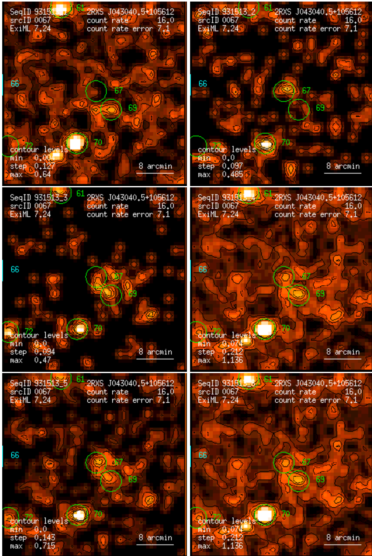
Figure 67: RASS 931513: detection 0067: band rate images, Gaussian filter: (1) PSPC channels 11 – 41, (2) 52 – 90, (3) 91 – 201, (4) 11 – 235, (5) 52 – 201, (6) 11 – 201. Broad band rates in counts/ks. Band rate contour levels in counts/ks/arcmin 2 .
