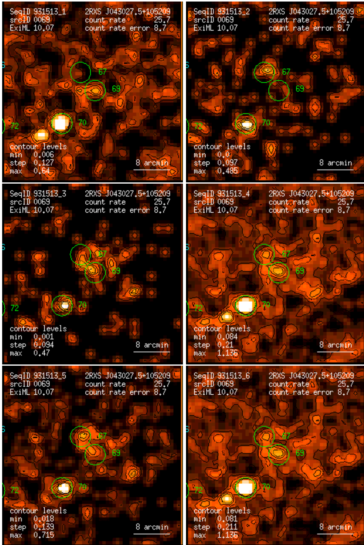
Figure 69: RASS 931513: detection 0069: band rate images, Gaussian filter: (1) PSPC channels 11 – 41, (2) 52 – 90, (3) 91 – 201, (4) 11 – 235, (5) 52 – 201, (6) 11 – 201. Broad band rates in counts/ks. Band rate contour levels in counts/ks/arcmin 2 .
