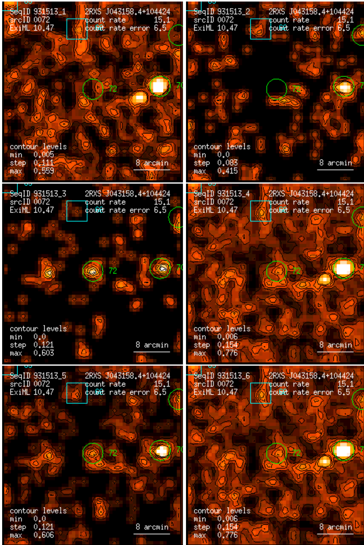
Figure 72: RASS 931513: detection 0072: band rate images, Gaussian filter: (1) PSPC channels 11 – 41, (2) 52 – 90, (3) 91 – 201, (4) 11 – 235, (5) 52 – 201, (6) 11 – 201. Broad band rates in counts/ks. Band rate contour levels in counts/ks/arcmin 2 .
