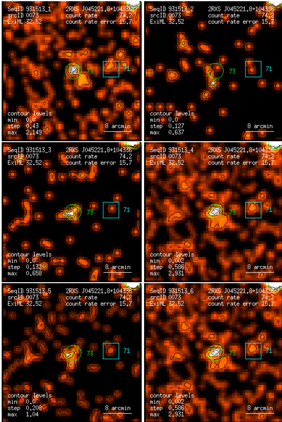
Figure 73: RASS 931513: detection 0073: band rate images, Gaussian filter: (1) PSPC channels 11 – 41, (2) 52 – 90, (3) 91 – 201, (4) 11 – 235, (5) 52 – 201, (6) 11 – 201. Broad band rates in counts/ks. Band rate contour levels in counts/ks/arcmin 2 .
