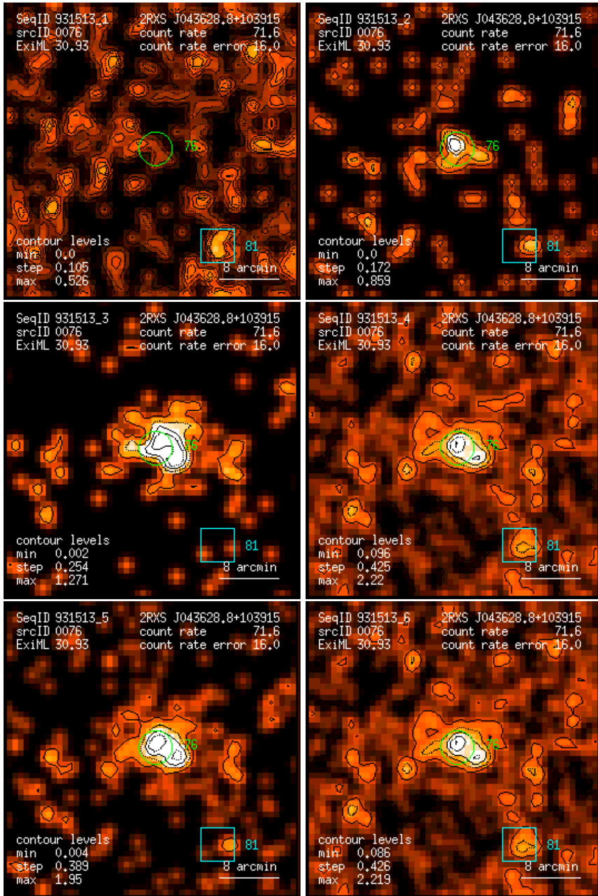
Figure 76: RASS 931513: detection 0076: band rate images, Gaussian filter: (1) PSPC channels 11 – 41, (2) 52 – 90, (3) 91 – 201, (4) 11 – 235, (5) 52 – 201, (6) 11 – 201. Broad band rates in counts/ks. Band rate contour levels in counts/ks/arcmin 2 .
