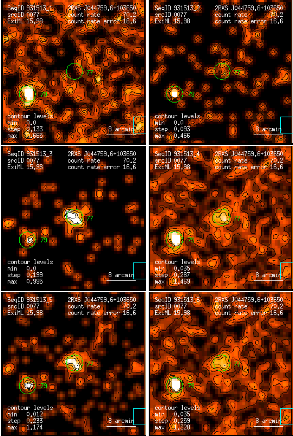
Figure 77: RASS 931513: detection 0077: band rate images, Gaussian filter: (1) PSPC channels 11 – 41, (2) 52 – 90, (3) 91 – 201, (4) 11 – 235, (5) 52 – 201, (6) 11 – 201. Broad band rates in counts/ks. Band rate contour levels in counts/ks/arcmin 2 .
