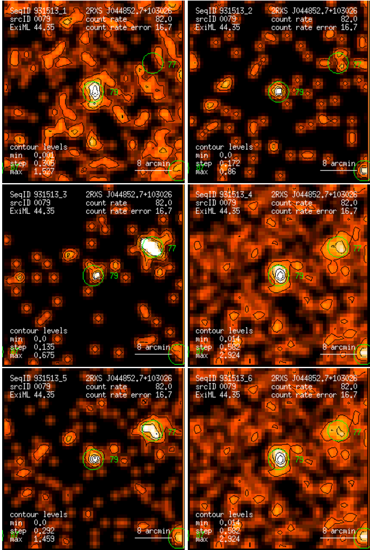
Figure 79: RASS 931513: detection 0079: band rate images, Gaussian filter: (1) PSPC channels 11 – 41, (2) 52 – 90, (3) 91 – 201, (4) 11 – 235, (5) 52 – 201, (6) 11 – 201. Broad band rates in counts/ks. Band rate contour levels in counts/ks/arcmin 2 .
