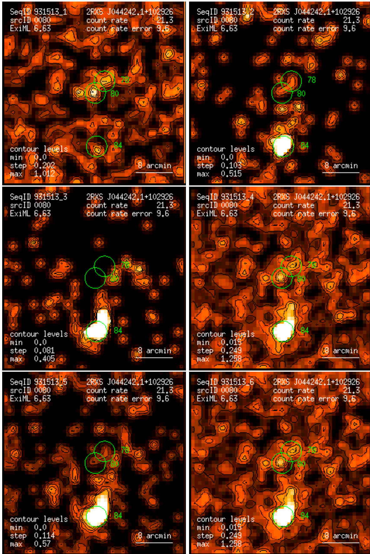
Figure 80: RASS 931513: detection 0080: band rate images, Gaussian filter: (1) PSPC channels 11 – 41, (2) 52 – 90, (3) 91 – 201, (4) 11 – 235, (5) 52 – 201, (6) 11 – 201. Broad band rates in counts/ks. Band rate contour levels in counts/ks/arcmin 2 .
