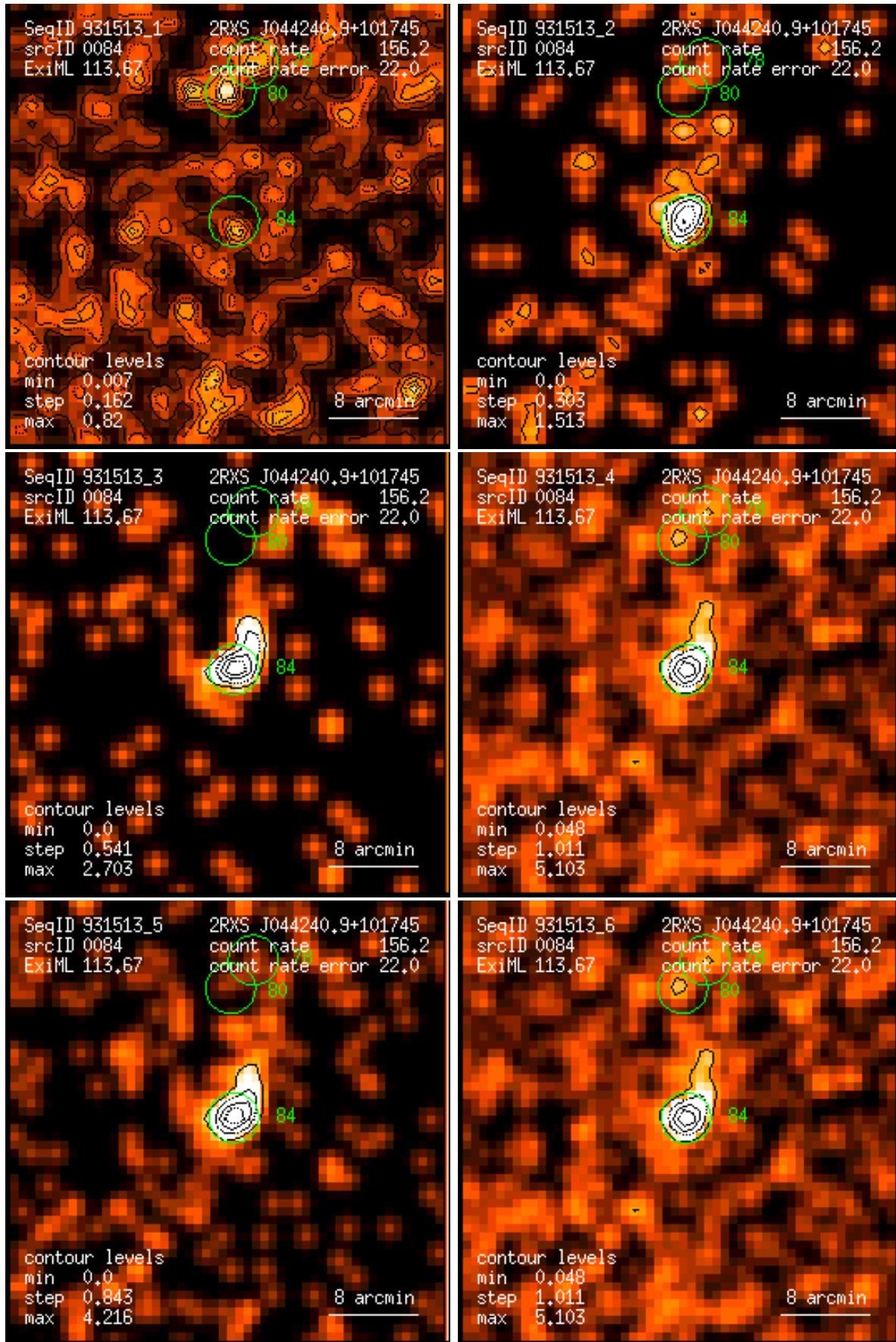
Figure 84: RASS 931513: detection 0084: band rate images, Gaussian filter: (1) PSPC channels 11 – 41, (2) 52 – 90, (3) 91 – 201, (4) 11 – 235, (5) 52 – 201, (6) 11 – 201. Broad band rates in counts/ks. Band rate contour levels in counts/ks/arcmin 2 .
