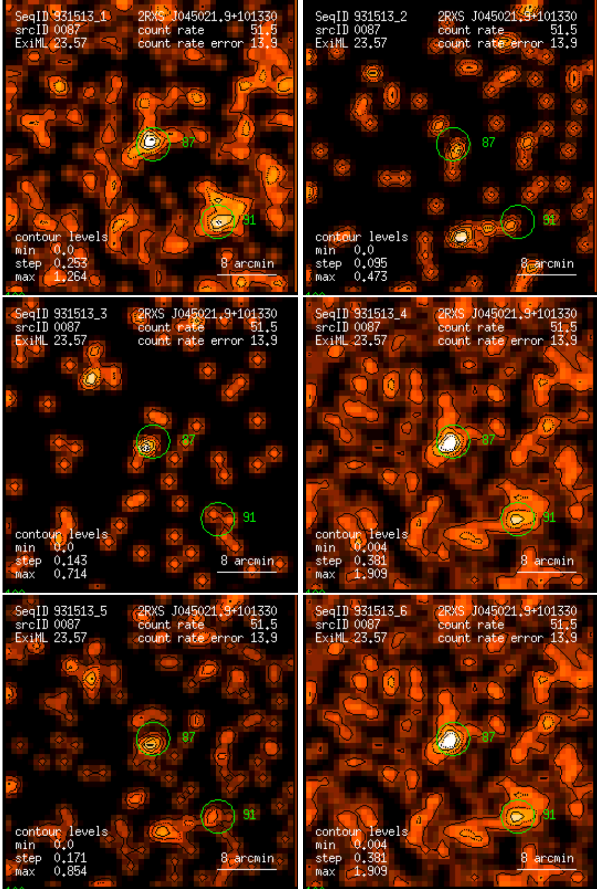
Figure 87: RASS 931513: detection 0087: band rate images, Gaussian filter: (1) PSPC channels 11 – 41, (2) 52 – 90, (3) 91 – 201, (4) 11 – 235, (5) 52 – 201, (6) 11 – 201. Broad band rates in counts/ks. Band rate contour levels in counts/ks/arcmin 2 .
