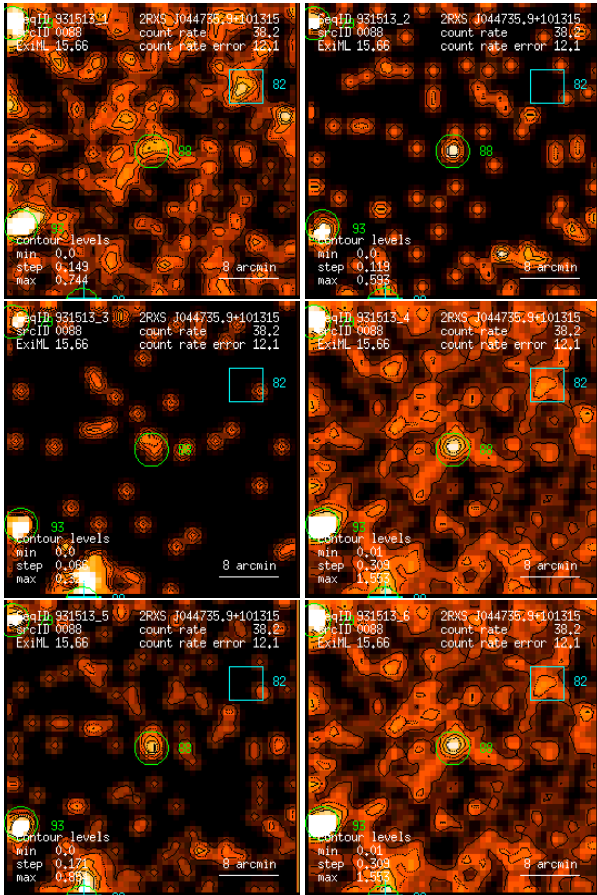
Figure 88: RASS 931513: detection 0088: band rate images, Gaussian filter: (1) PSPC channels 11 – 41, (2) 52 – 90, (3) 91 – 201, (4) 11 – 235, (5) 52 – 201, (6) 11 – 201. Broad band rates in counts/ks. Band rate contour levels in counts/ks/arcmin 2 .
