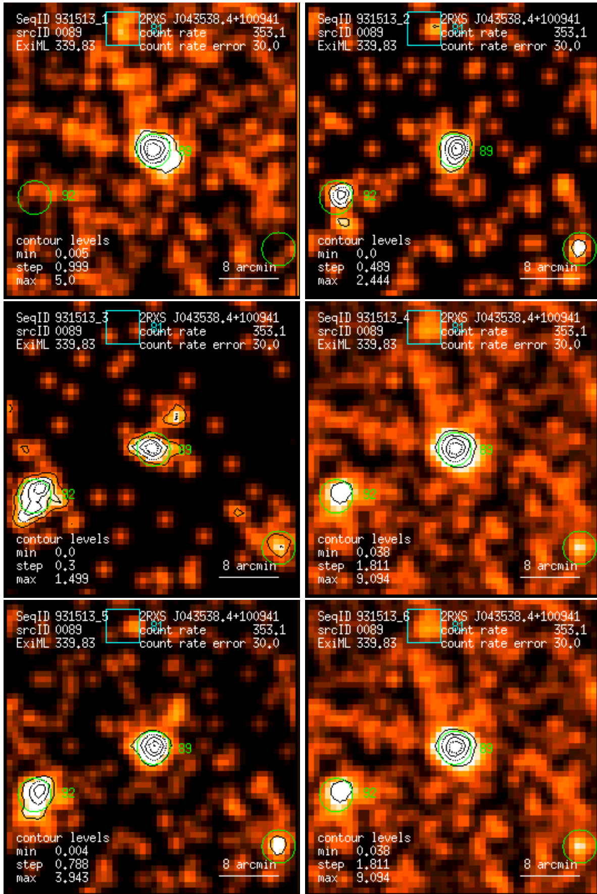
Figure 89: RASS 931513: detection 0089: band rate images, Gaussian filter: (1) PSPC channels 11 – 41, (2) 52 – 90, (3) 91 – 201, (4) 11 – 235, (5) 52 – 201, (6) 11 – 201. Broad band rates in counts/ks. Band rate contour levels in counts/ks/arcmin 2 .
