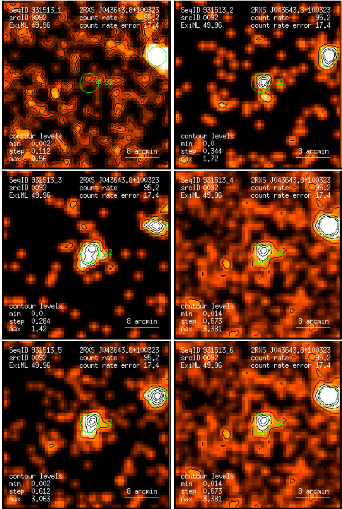
Figure 92: RASS 931513: detection 0092: band rate images, Gaussian filter: (1) PSPC channels 11 – 41, (2) 52 – 90, (3) 91 – 201, (4) 11 – 235, (5) 52 – 201, (6) 11 – 201. Broad band rates in counts/ks. Band rate contour levels in counts/ks/arcmin 2 .
