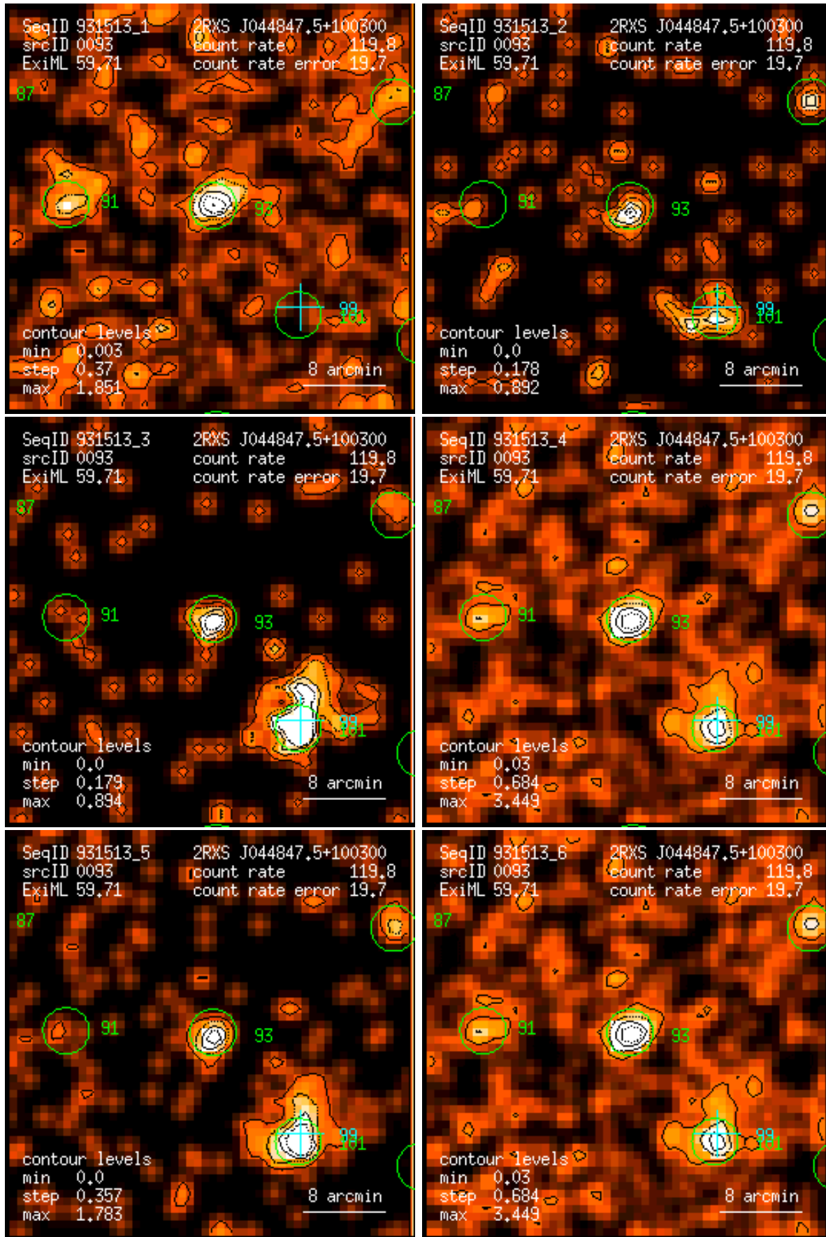
Figure 93: RASS 931513: detection 0093: band rate images, Gaussian filter: (1) PSPC channels 11 – 41, (2) 52 – 90, (3) 91 – 201, (4) 11 – 235, (5) 52 – 201, (6) 11 – 201. Broad band rates in counts/ks. Band rate contour levels in counts/ks/arcmin 2 .
