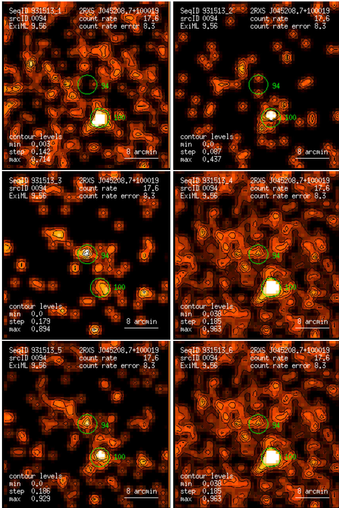
Figure 94: RASS 931513: detection 0094: band rate images, Gaussian filter: (1) PSPC channels 11 – 41, (2) 52 – 90, (3) 91 – 201, (4) 11 – 235, (5) 52 – 201, (6) 11 – 201. Broad band rates in counts/ks. Band rate contour levels in counts/ks/arcmin 2 .
