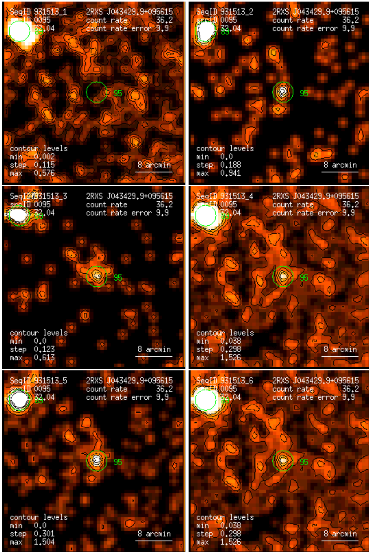
Figure 95: RASS 931513: detection 0095: band rate images, Gaussian filter: (1) PSPC channels 11 – 41, (2) 52 – 90, (3) 91 – 201, (4) 11 – 235, (5) 52 – 201, (6) 11 – 201. Broad band rates in counts/ks. Band rate contour levels in counts/ks/arcmin 2 .
