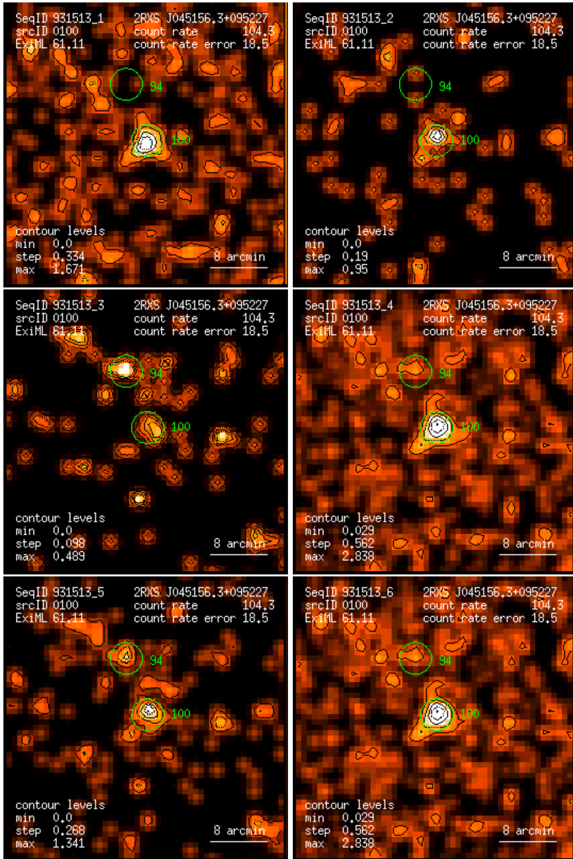
Figure 100: RASS 931513: detection 0100: band rate images, Gaussian filter: (1) PSPC channels 11 – 41, (2) 52 – 90, (3) 91 – 201, (4) 11 – 235, (5) 52 – 201, (6) 11 – 201. Broad band rates in counts/ks. Band rate contour levels in counts/ks/arcmin 2 .
