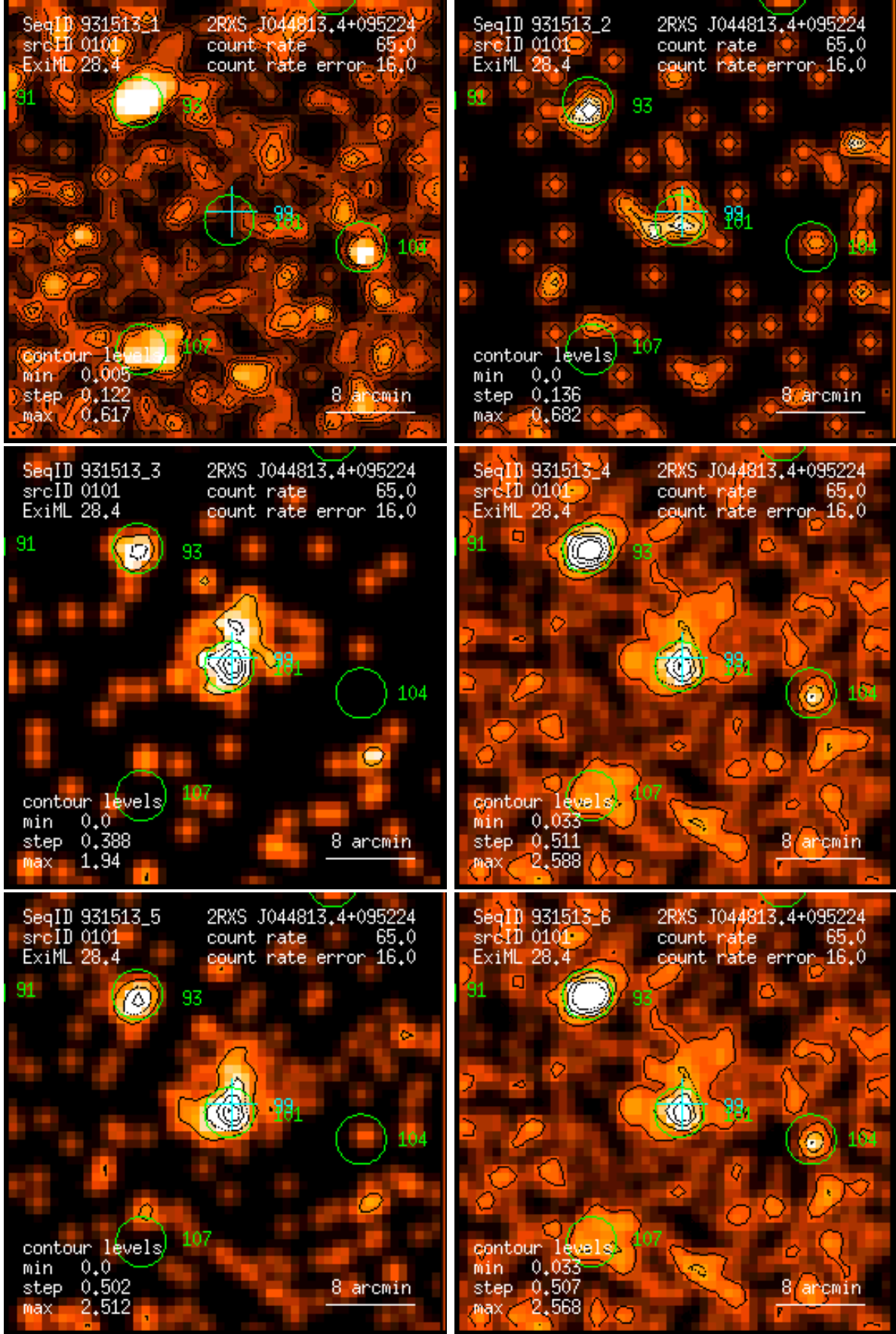
Figure 101: RASS 931513: detection 0101: band rate images, Gaussian filter: (1) PSPC channels 11 – 41, (2) 52 – 90, (3) 91 – 201, (4) 11 – 235, (5) 52 – 201, (6) 11 – 201. Broad band rates in counts/ks. Band rate contour levels in counts/ks/arcmin 2 .
