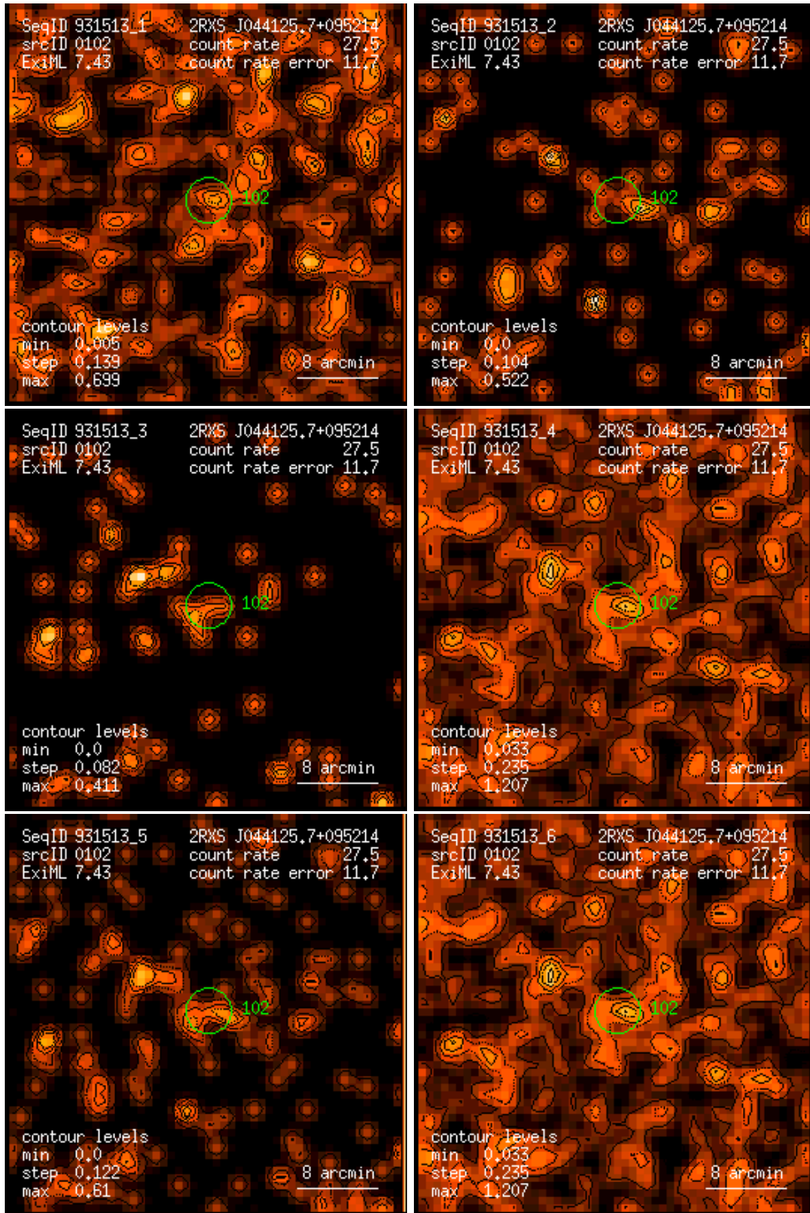
Figure 102: RASS 931513: detection 0102: band rate images, Gaussian filter: (1) PSPC channels 11 – 41, (2) 52 – 90, (3) 91 – 201, (4) 11 – 235, (5) 52 – 201, (6) 11 – 201. Broad band rates in counts/ks. Band rate contour levels in counts/ks/arcmin 2 .
