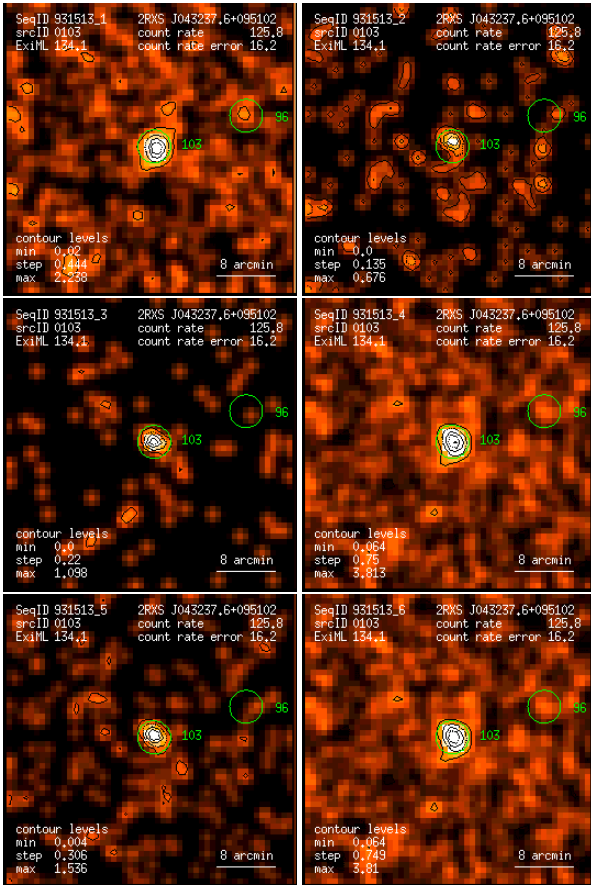
Figure 103: RASS 931513: detection 0103: band rate images, Gaussian filter: (1) PSPC channels 11 – 41, (2) 52 – 90, (3) 91 – 201, (4) 11 – 235, (5) 52 – 201, (6) 11 – 201. Broad band rates in counts/ks. Band rate contour levels in counts/ks/arcmin 2 .
