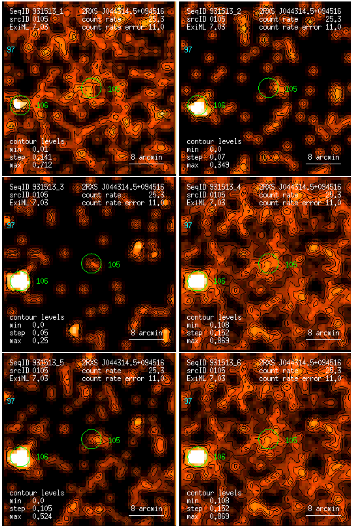
Figure 105: RASS 931513: detection 0105: band rate images, Gaussian filter: (1) PSPC channels 11 – 41, (2) 52 – 90, (3) 91 – 201, (4) 11 – 235, (5) 52 – 201, (6) 11 – 201. Broad band rates in counts/ks. Band rate contour levels in counts/ks/arcmin 2 .
