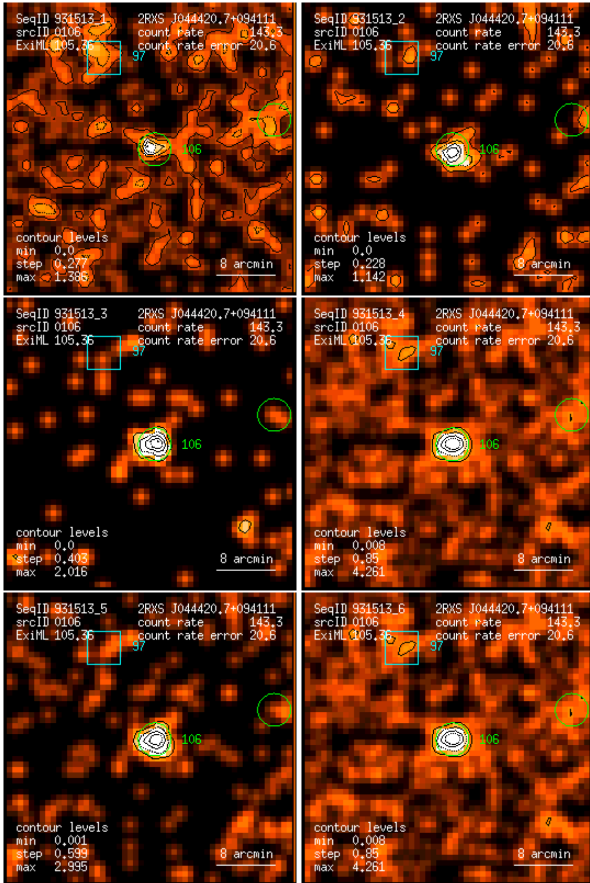
Figure 106: RASS 931513: detection 0106: band rate images, Gaussian filter: (1) PSPC channels 11 – 41, (2) 52 – 90, (3) 91 – 201, (4) 11 – 235, (5) 52 – 201, (6) 11 – 201. Broad band rates in counts/ks. Band rate contour levels in counts/ks/arcmin 2 .
