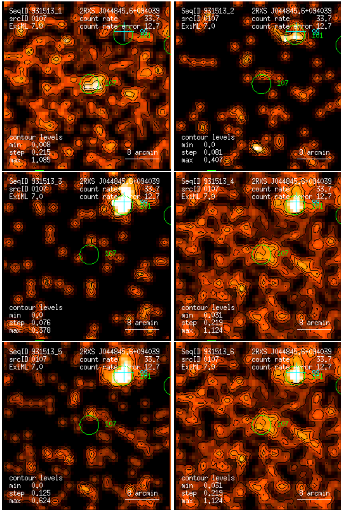
Figure 107: RASS 931513: detection 0107: band rate images, Gaussian filter: (1) PSPC channels 11 – 41, (2) 52 – 90, (3) 91 – 201, (4) 11 – 235, (5) 52 – 201, (6) 11 – 201. Broad band rates in counts/ks. Band rate contour levels in counts/ks/arcmin 2 .
