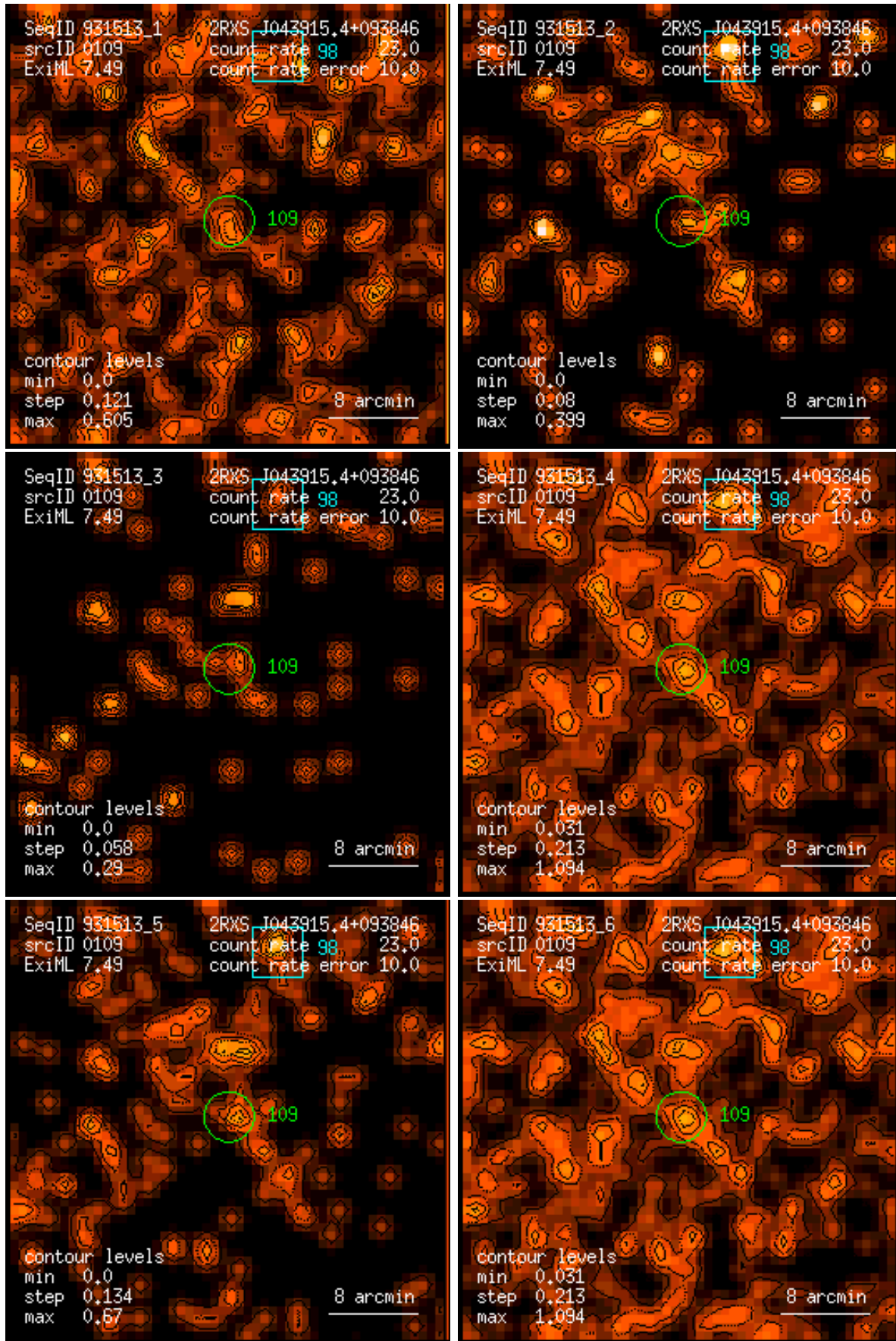
Figure 109: RASS 931513: detection 0109: band rate images, Gaussian filter: (1) PSPC channels 11 – 41, (2) 52 – 90, (3) 91 – 201, (4) 11 – 235, (5) 52 – 201, (6) 11 – 201. Broad band rates in counts/ks. Band rate contour levels in counts/ks/arcmin 2 .
