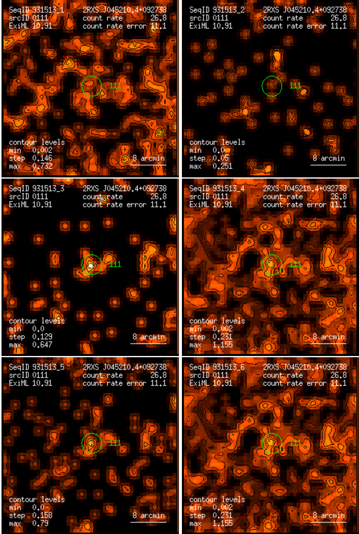
Figure 111: RASS 931513: detection 0111: band rate images, Gaussian filter: (1) PSPC channels 11 – 41, (2) 52 – 90, (3) 91 – 201, (4) 11 – 235, (5) 52 – 201, (6) 11 – 201. Broad band rates in counts/ks. Band rate contour levels in counts/ks/arcmin 2 .
