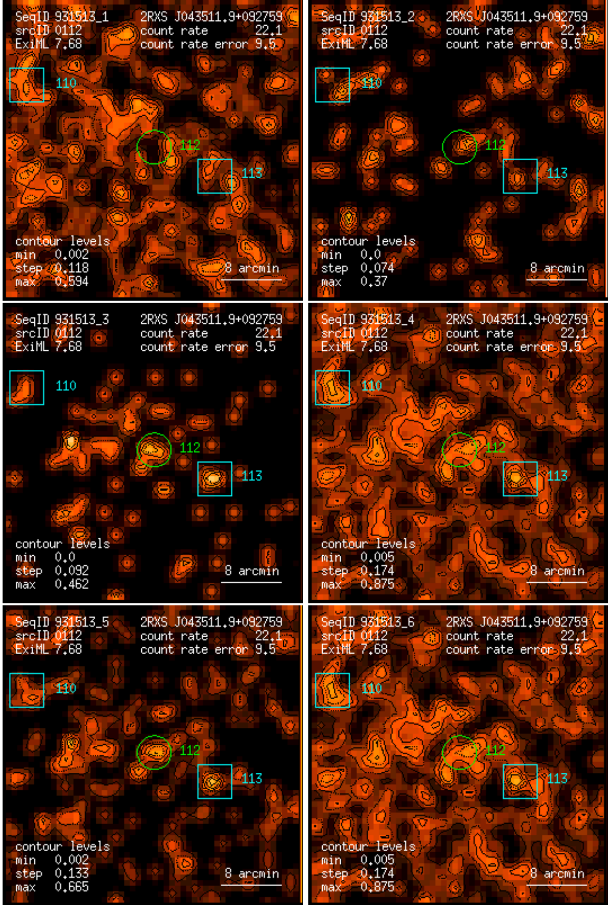
Figure 112: RASS 931513: detection 0112: band rate images, Gaussian filter: (1) PSPC channels 11 – 41, (2) 52 – 90, (3) 91 – 201, (4) 11 – 235, (5) 52 – 201, (6) 11 – 201. Broad band rates in counts/ks. Band rate contour levels in counts/ks/arcmin 2 .
