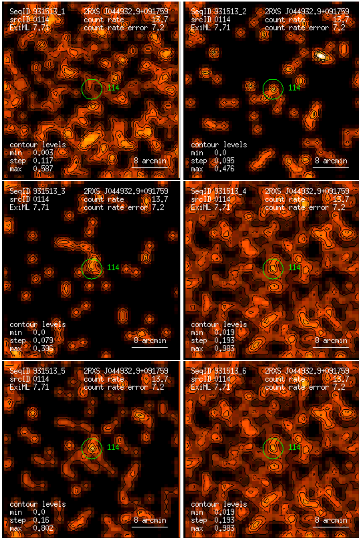
Figure 114: RASS 931513: detection 0114: band rate images, Gaussian filter: (1) PSPC channels 11 – 41, (2) 52 – 90, (3) 91 – 201, (4) 11 – 235, (5) 52 – 201, (6) 11 – 201. Broad band rates in counts/ks. Band rate contour levels in counts/ks/arcmin 2 .
