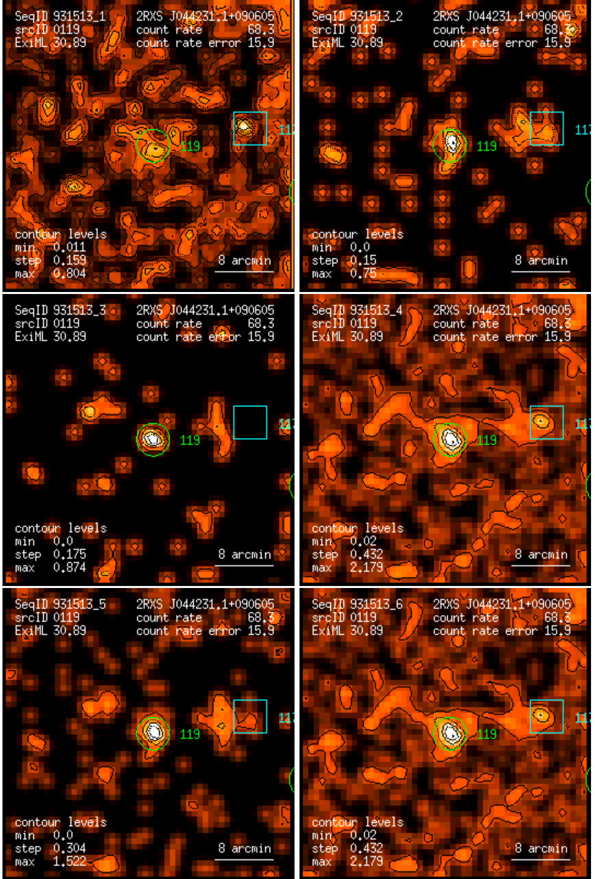
Figure 119: RASS 931513: detection 0119: band rate images, Gaussian filter: (1) PSPC channels 11 – 41, (2) 52 – 90, (3) 91 – 201, (4) 11 – 235, (5) 52 – 201, (6) 11 – 201. Broad band rates in counts/ks. Band rate contour levels in counts/ks/arcmin 2 .
