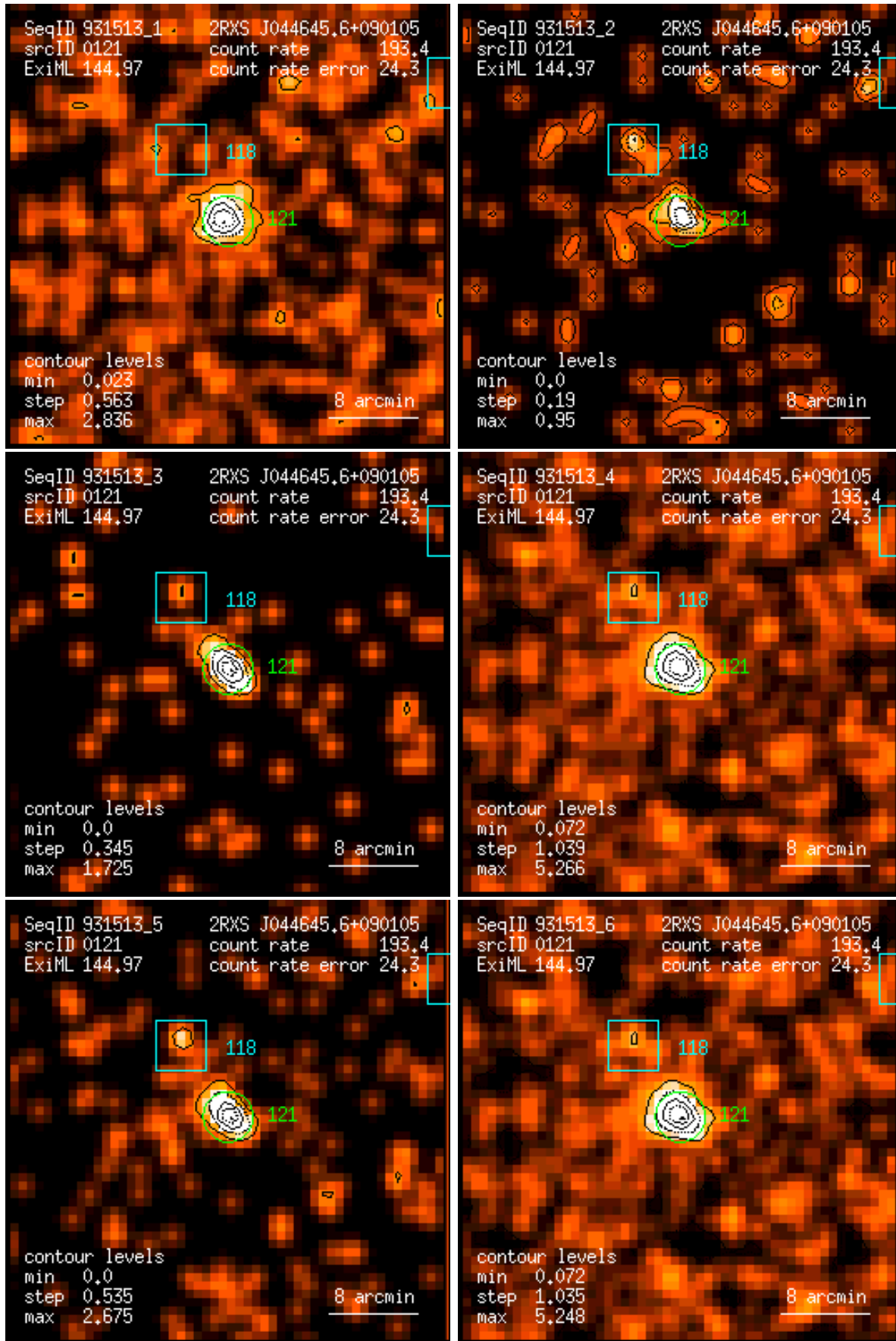
Figure 121: RASS 931513: detection 0121: band rate images, Gaussian filter: (1) PSPC channels 11 – 41, (2) 52 – 90, (3) 91 – 201, (4) 11 – 235, (5) 52 – 201, (6) 11 – 201. Broad band rates in counts/ks. Band rate contour levels in counts/ks/arcmin 2 .
