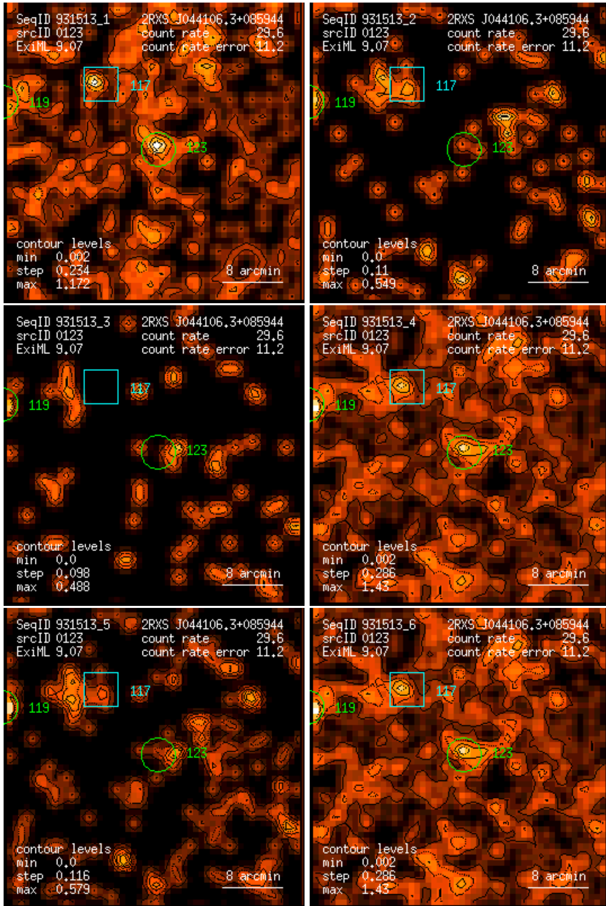
Figure 123: RASS 931513: detection 0123: band rate images, Gaussian filter: (1) PSPC channels 11 – 41, (2) 52 – 90, (3) 91 – 201, (4) 11 – 235, (5) 52 – 201, (6) 11 – 201. Broad band rates in counts/ks. Band rate contour levels in counts/ks/arcmin 2 .
