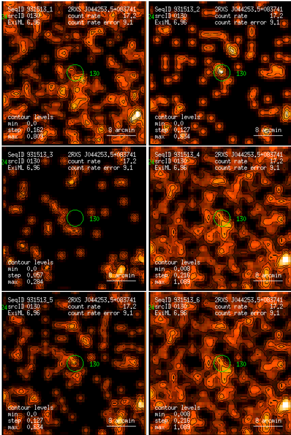
Figure 130: RASS 931513: detection 0130: band rate images, Gaussian filter: (1) PSPC channels 11 – 41, (2) 52 – 90, (3) 91 – 201, (4) 11 – 235, (5) 52 – 201, (6) 11 – 201. Broad band rates in counts/ks. Band rate contour levels in counts/ks/arcmin 2 .
