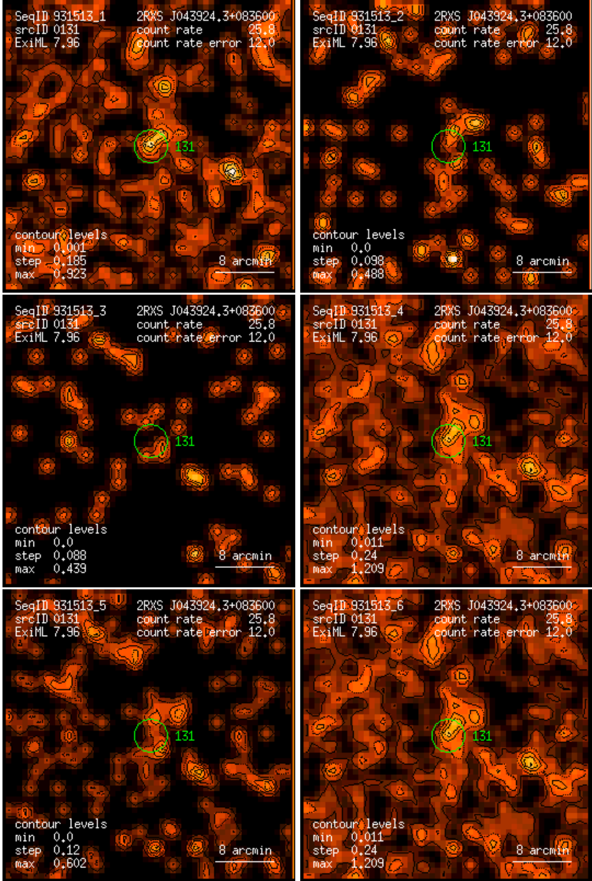
Figure 131: RASS 931513: detection 0131: band rate images, Gaussian filter: (1) PSPC channels 11 – 41, (2) 52 – 90, (3) 91 – 201, (4) 11 – 235, (5) 52 – 201, (6) 11 – 201. Broad band rates in counts/ks. Band rate contour levels in counts/ks/arcmin 2 .
