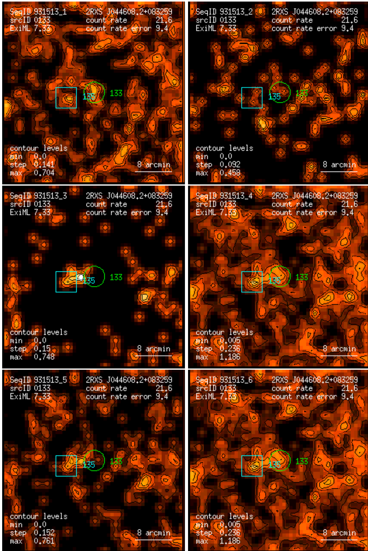
Figure 133: RASS 931513: detection 0133: band rate images, Gaussian filter: (1) PSPC channels 11 – 41, (2) 52 – 90, (3) 91 – 201, (4) 11 – 235, (5) 52 – 201, (6) 11 – 201. Broad band rates in counts/ks. Band rate contour levels in counts/ks/arcmin 2 .
