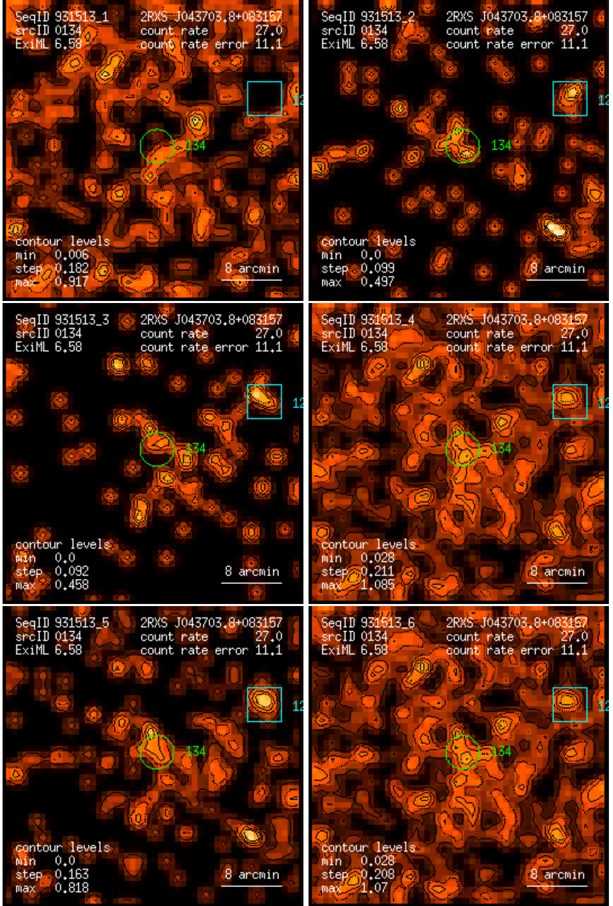
Figure 134: RASS 931513: detection 0134: band rate images, Gaussian filter: (1) PSPC channels 11 – 41, (2) 52 – 90, (3) 91 – 201, (4) 11 – 235, (5) 52 – 201, (6) 11 – 201. Broad band rates in counts/ks. Band rate contour levels in counts/ks/arcmin 2 .
