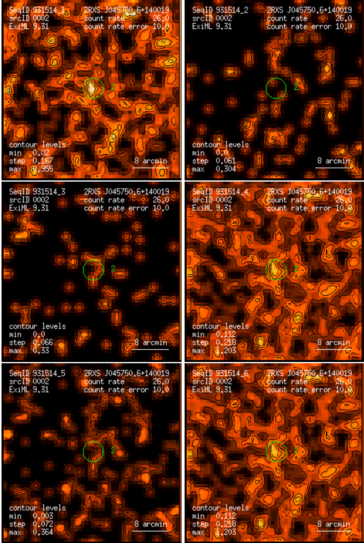
Figure 2: RASS 931514: detection 0002: band rate images, Gaussian filter: (1) PSPC channels 11 – 41, (2) 52 – 90, (3) 91 – 201, (4) 11 – 235, (5) 52 – 201, (6) 11 – 201. Broad band rates in counts/ks. Band rate contour levels in counts/ks/arcmin 2 .
