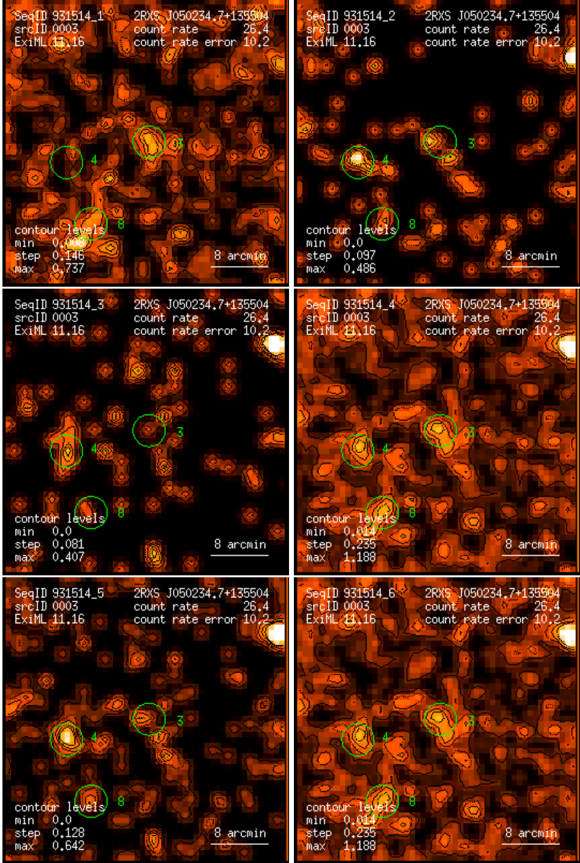
Figure 3: RASS 931514: detection 0003: band rate images, Gaussian filter: (1) PSPC channels 11 – 41, (2) 52 – 90, (3) 91 – 201, (4) 11 – 235, (5) 52 – 201, (6) 11 – 201. Broad band rates in counts/ks. Band rate contour levels in counts/ks/arcmin 2 .
