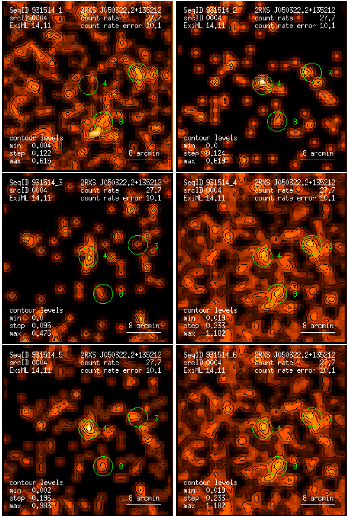
Figure 4: RASS 931514: detection 0004: band rate images, Gaussian filter: (1) PSPC channels 11 – 41, (2) 52 – 90, (3) 91 – 201, (4) 11 – 235, (5) 52 – 201, (6) 11 – 201. Broad band rates in counts/ks. Band rate contour levels in counts/ks/arcmin 2 .
