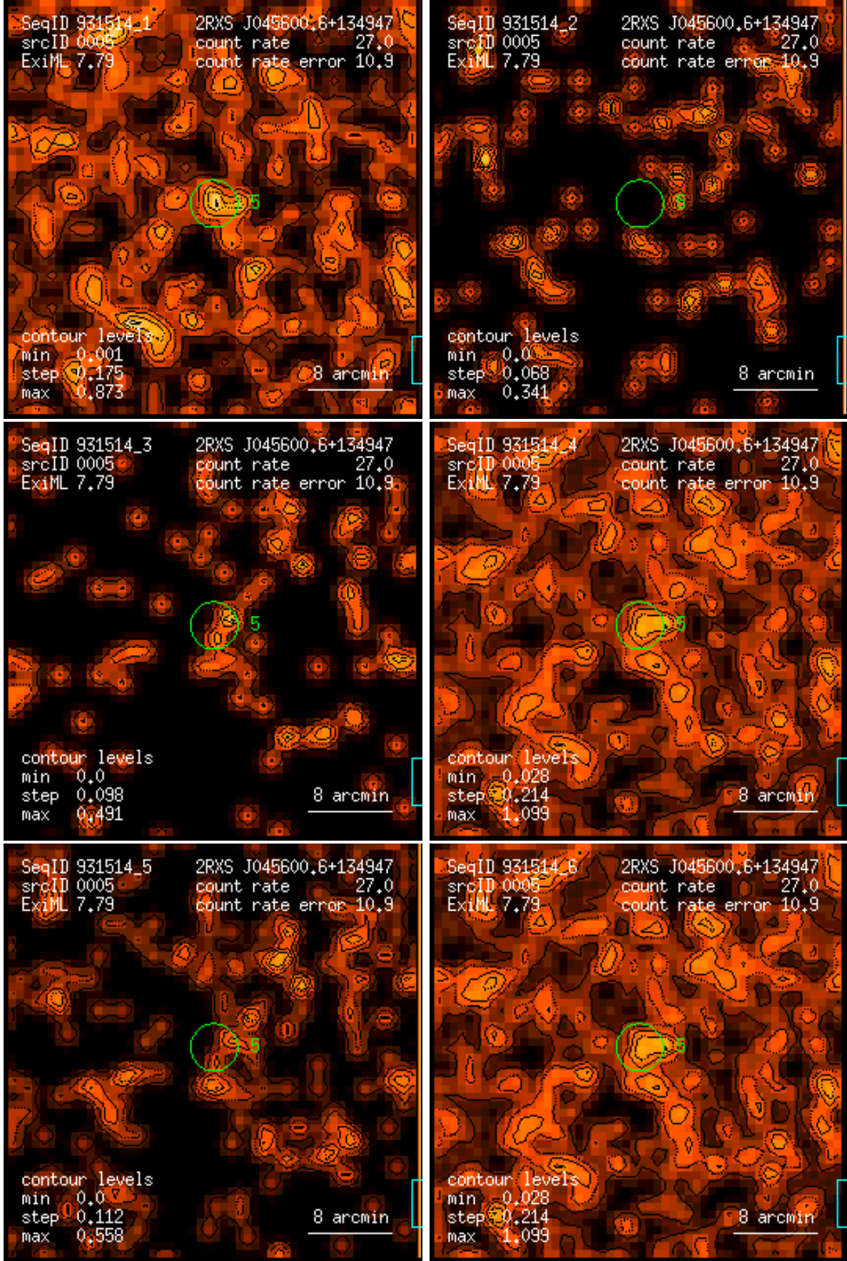
Figure 5: RASS 931514: detection 0005: band rate images, Gaussian filter: (1) PSPC channels 11 – 41, (2) 52 – 90, (3) 91 – 201, (4) 11 – 235, (5) 52 – 201, (6) 11 – 201. Broad band rates in counts/ks. Band rate contour levels in counts/ks/arcmin 2 .
