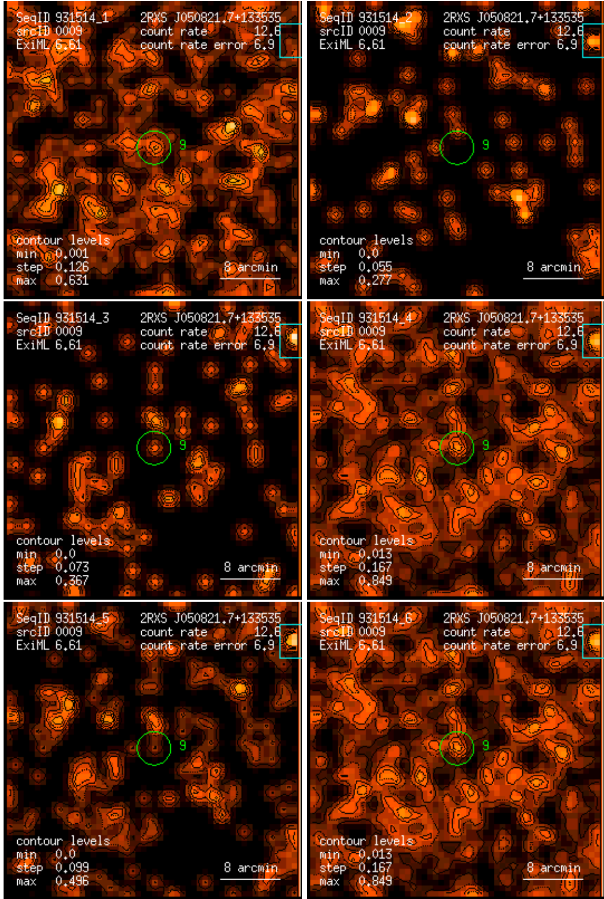
Figure 9: RASS 931514: detection 0009: band rate images, Gaussian filter: (1) PSPC channels 11 – 41, (2) 52 – 90, (3) 91 – 201, (4) 11 – 235, (5) 52 – 201, (6) 11 – 201. Broad band rates in counts/ks. Band rate contour levels in counts/ks/arcmin 2 .
