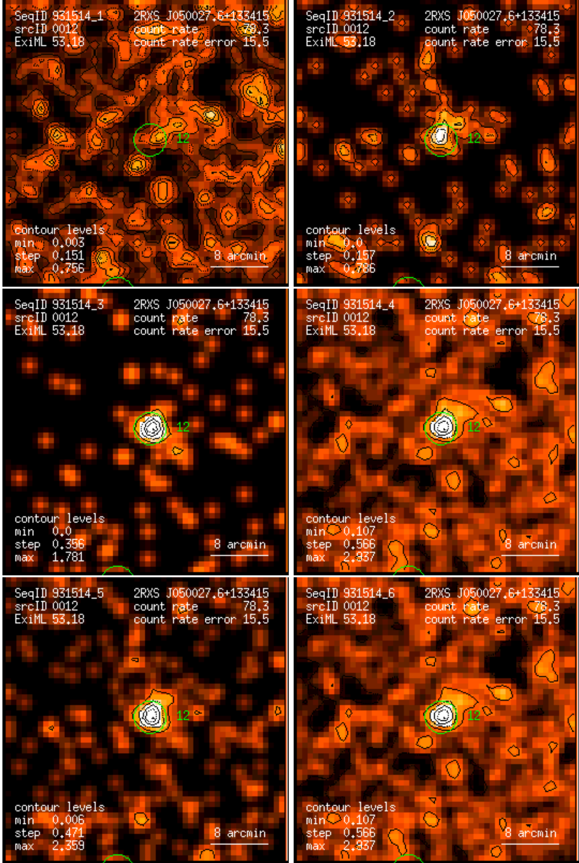
Figure 12: RASS 931514: detection 0012: band rate images, Gaussian filter: (1) PSPC channels 11 – 41, (2) 52 – 90, (3) 91 – 201, (4) 11 – 235, (5) 52 – 201, (6) 11 – 201. Broad band rates in counts/ks. Band rate contour levels in counts/ks/arcmin 2 .
