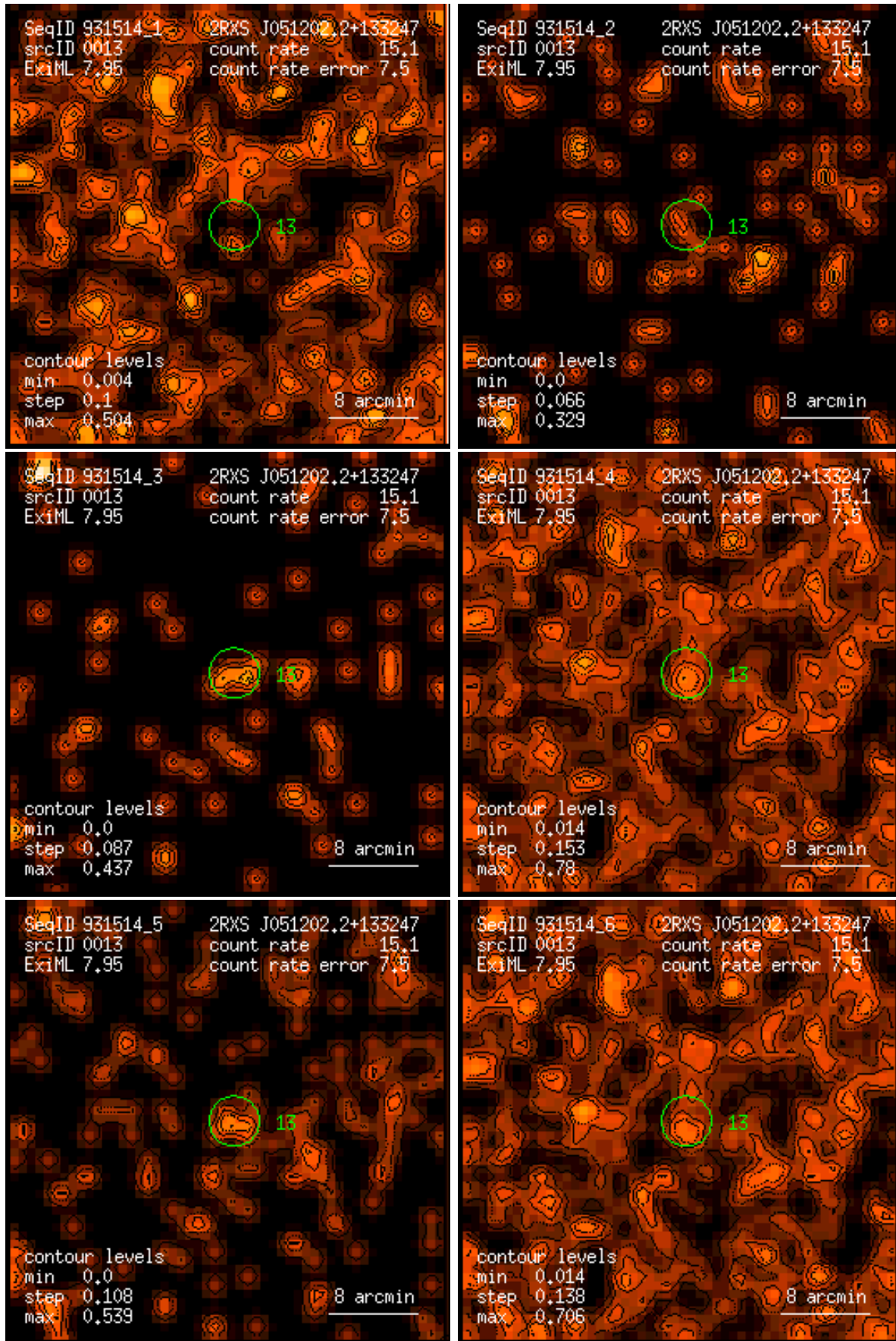
Figure 13: RASS 931514: detection 0013: band rate images, Gaussian filter: (1) PSPC channels 11 – 41, (2) 52 – 90, (3) 91 – 201, (4) 11 – 235, (5) 52 – 201, (6) 11 – 201. Broad band rates in counts/ks. Band rate contour levels in counts/ks/arcmin 2 .
