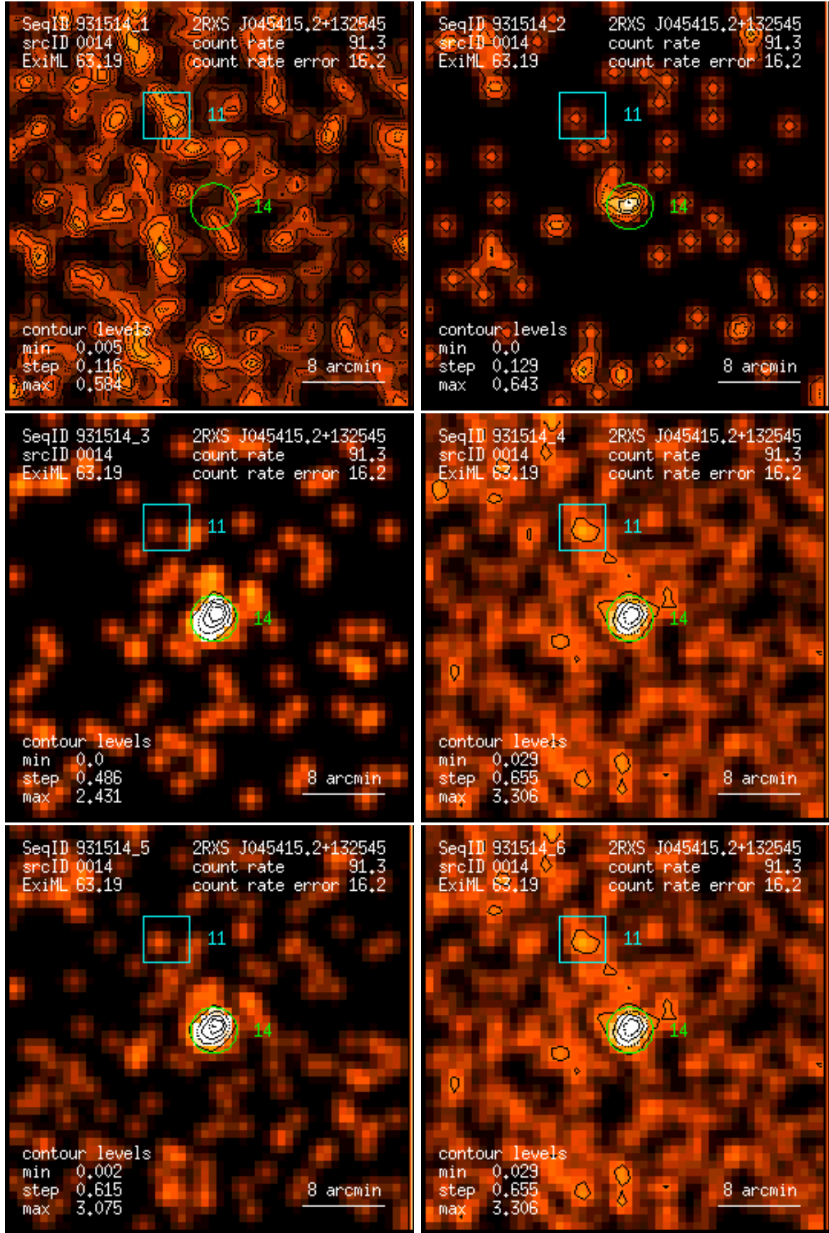
Figure 14: RASS 931514: detection 0014: band rate images, Gaussian filter: (1) PSPC channels 11 – 41, (2) 52 – 90, (3) 91 – 201, (4) 11 – 235, (5) 52 – 201, (6) 11 – 201. Broad band rates in counts/ks. Band rate contour levels in counts/ks/arcmin 2 .
