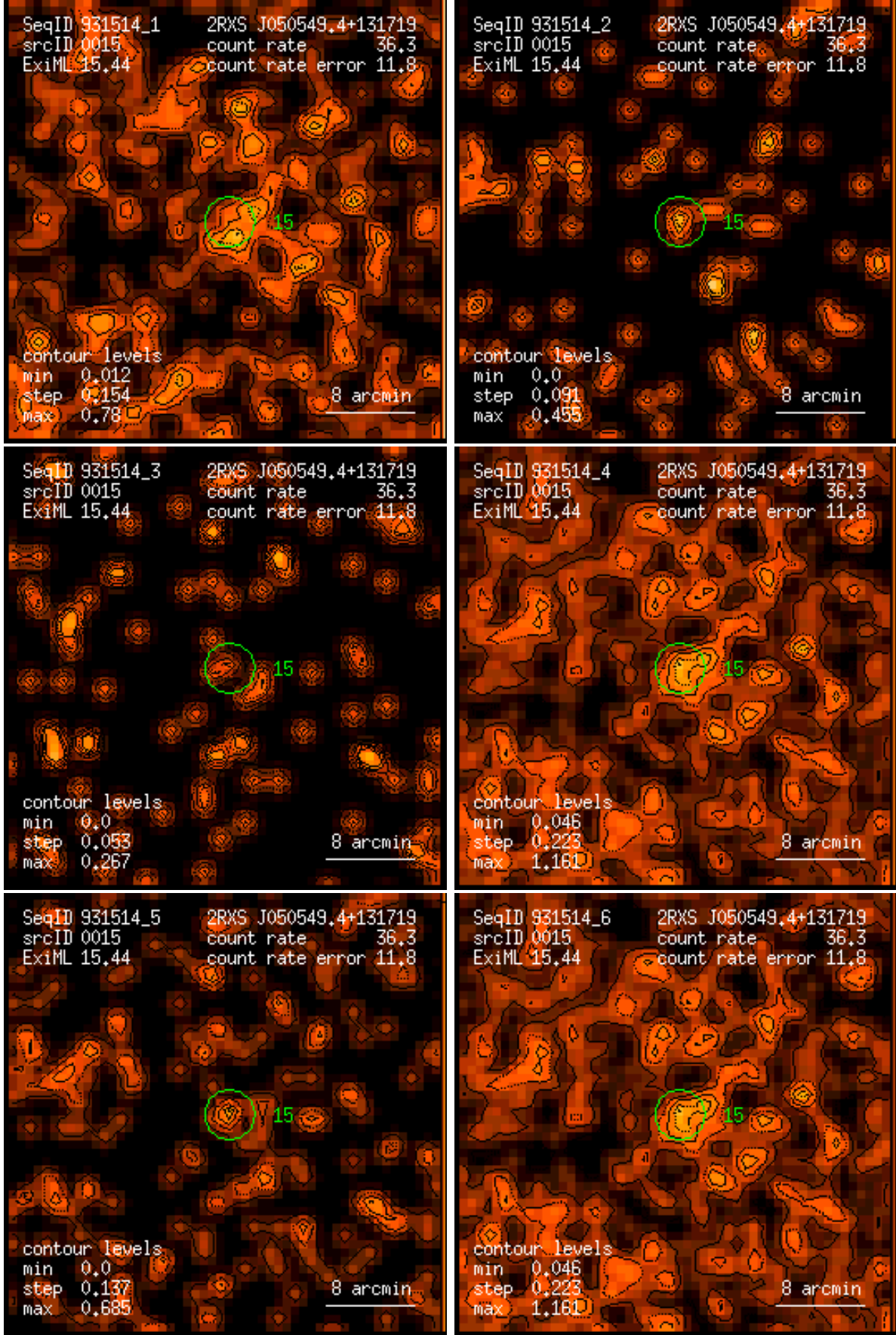
Figure 15: RASS 931514: detection 0015: band rate images, Gaussian filter: (1) PSPC channels 11 – 41, (2) 52 – 90, (3) 91 – 201, (4) 11 – 235, (5) 52 – 201, (6) 11 – 201. Broad band rates in counts/ks. Band rate contour levels in counts/ks/arcmin 2 .
