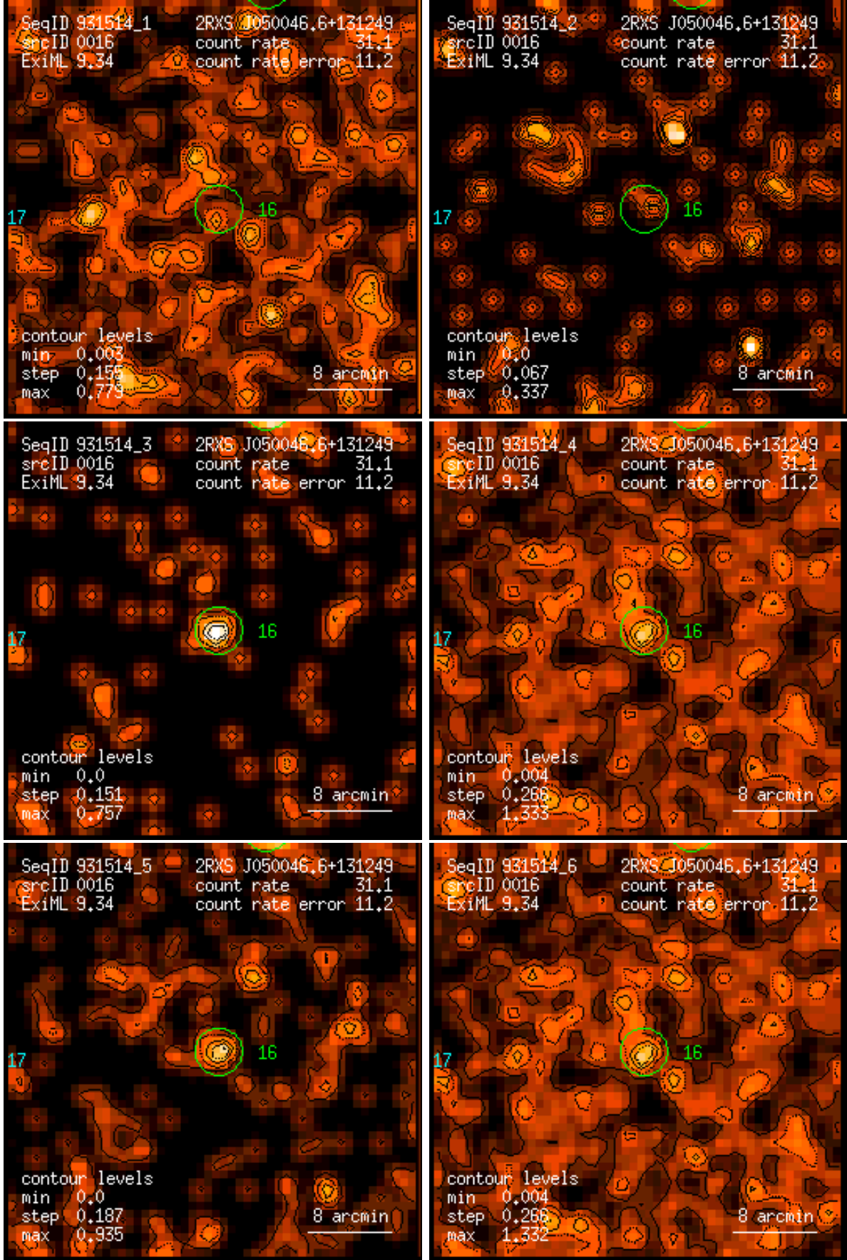
Figure 16: RASS 931514: detection 0016: band rate images, Gaussian filter: (1) PSPC channels 11 – 41, (2) 52 – 90, (3) 91 – 201, (4) 11 – 235, (5) 52 – 201, (6) 11 – 201. Broad band rates in counts/ks. Band rate contour levels in counts/ks/arcmin 2 .
