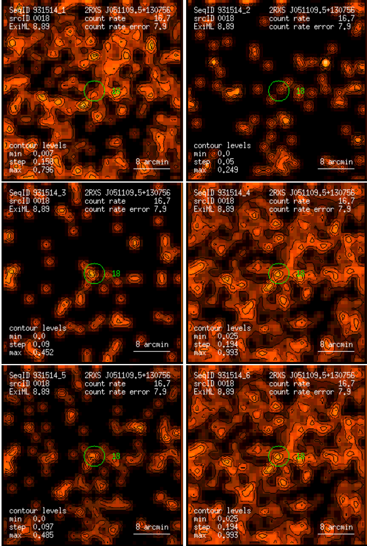
Figure 18: RASS 931514: detection 0018: band rate images, Gaussian filter: (1) PSPC channels 11 – 41, (2) 52 – 90, (3) 91 – 201, (4) 11 – 235, (5) 52 – 201, (6) 11 – 201. Broad band rates in counts/ks. Band rate contour levels in counts/ks/arcmin 2 .
